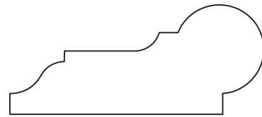
NM-0054 13/16"x1-7/8" PICTURE MOULDING
