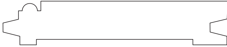
NM-0074 3/4"x3-13/16"
